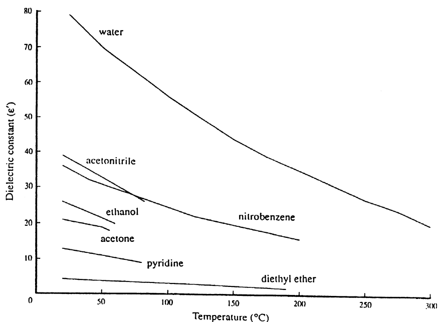
Figure 8. Plots of dielectric constants against temperature for various solvents [Strauss, C. R.; Trainor, R. W. Aust. J. Chem. , 1995 , 48 , 1665–1692, with the permission of CSIRO Publishing, Melbourne, Australia.]
